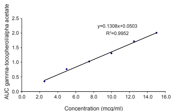
Figure 2. Calibration curve of standard gamma-tocopherol (2.5-15 \mu\text{g/ml} ).
