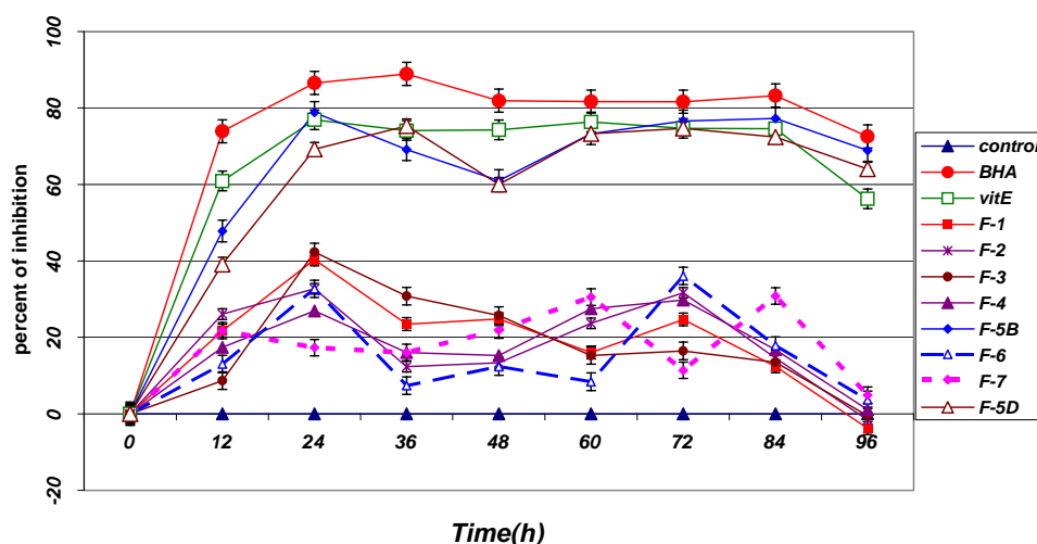
Figure 2. Antioxidant activity of different fractions of O. persica in comparison to negative and positive controls
