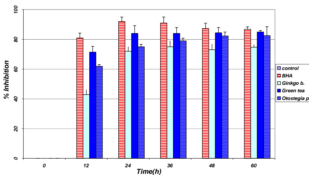
Figure 1. Antioxidant activity of methanolic extract of O.persica in comparison to negative and positive controls.
