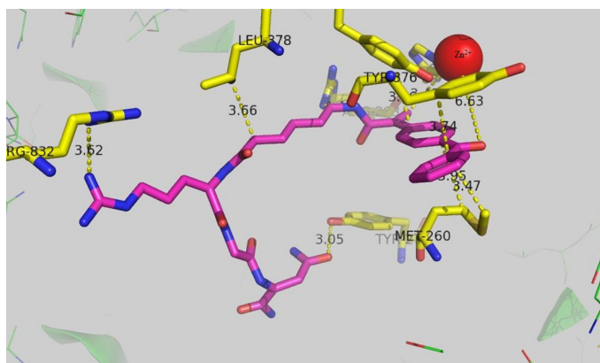
Figure 1. The docking result of ketoprofen-spacer-NGR with aminopeptidase N (PDB code: 2DQM).
