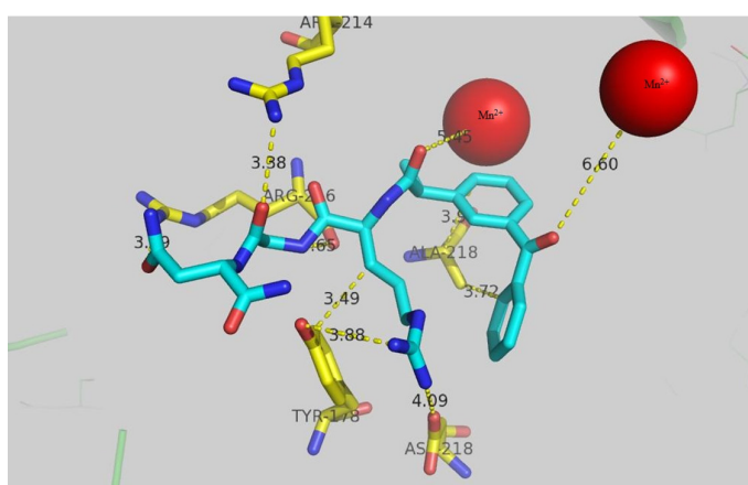
Figure 2. The docking result of ketoprofen-spacer-RGD with \alpha_v\beta_3 integrin (PDB code: 1L5G).
