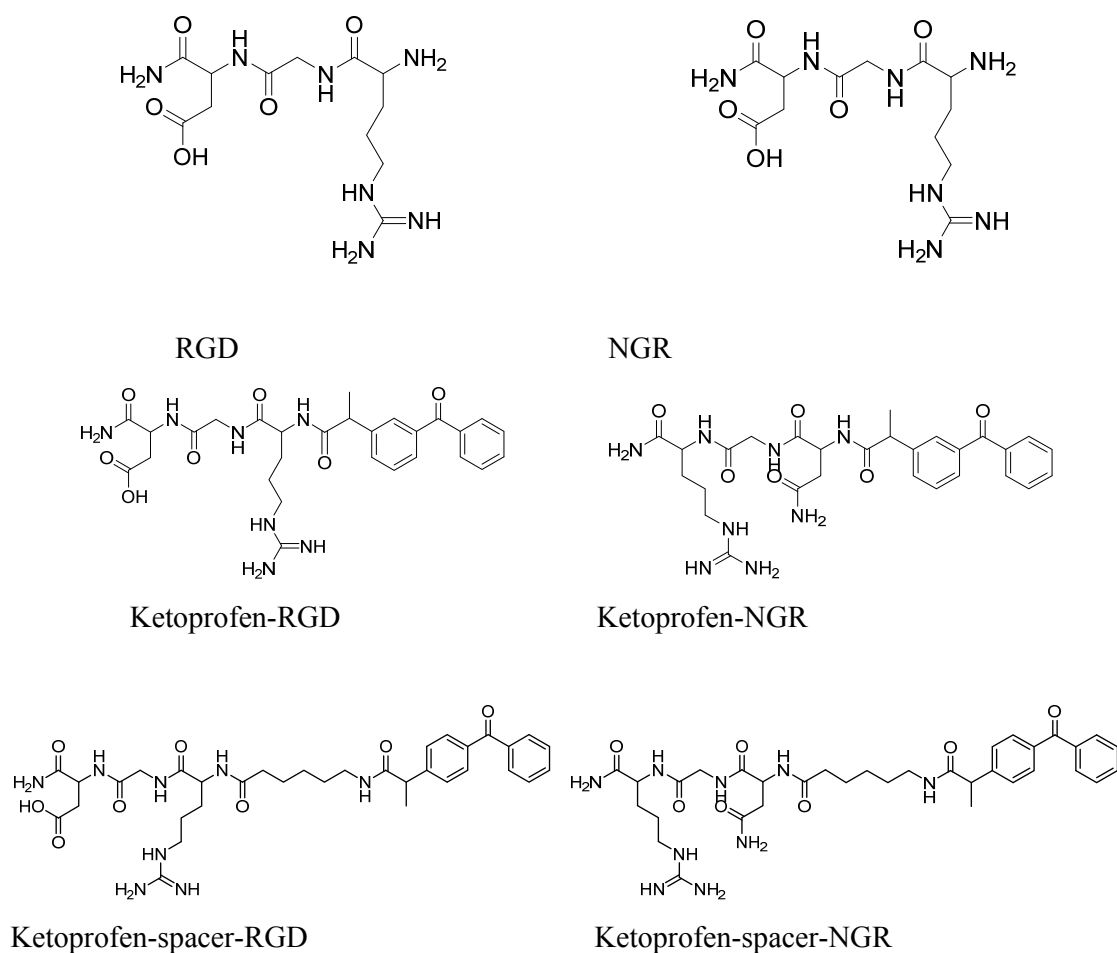
Scheme 3. Structure of all compounds.
