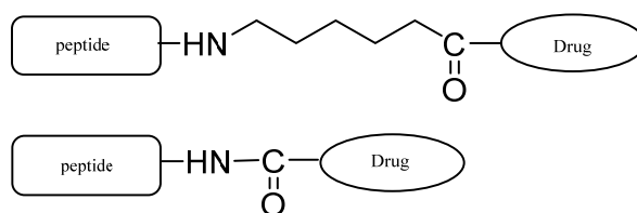
Scheme 1. Peptide-drug and peptide-spacer-drug conjugates. Peptide = RGD or NGR, Drug = ketoprofen.
