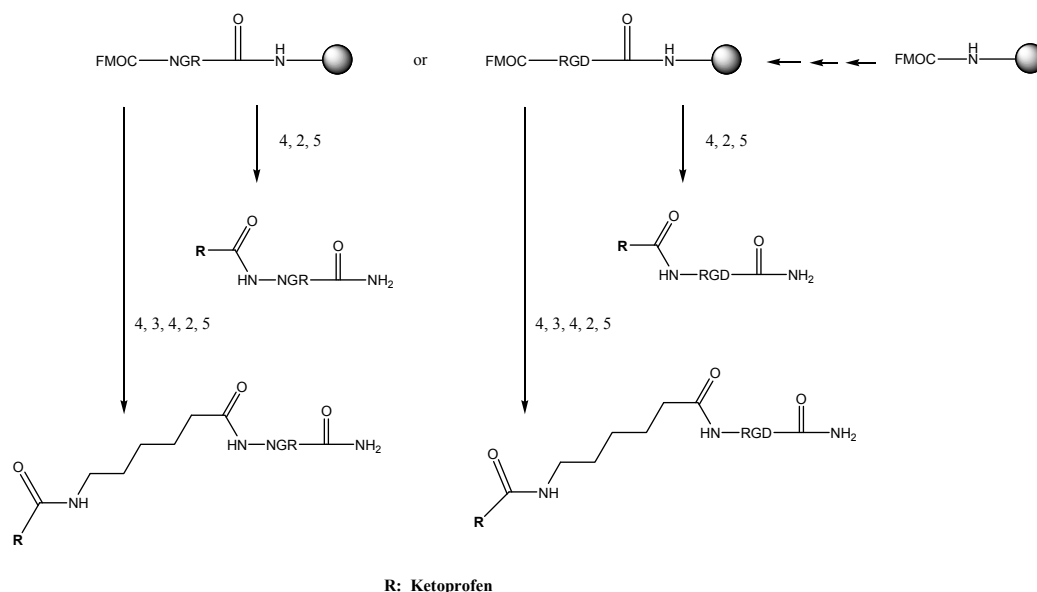
Scheme 2. Solid-phase peptide synthesis of RGD or NGR Drug conjugated, (1) solid phase peptide synthesis, (2) ketoprofen, HATU, DIEA, DMF, (3) fmoc-amino hexanoic acid, HATU, DIEA, DMF, (4) fmoc deprotection by Piperidine 20%, (5) cleavage by TFA, Thioanisol, p -cresol, TIS.
