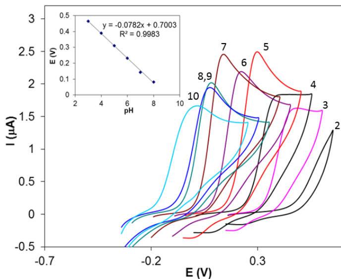
Figure 1. Cyclic voltammograms of 0.65 \mu\text{M} Hy-HCl in 0.1 M PBS at different pH values. Inset shows potential vs. pH curve.
