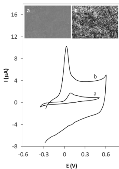
Figure 3. Cyclic voltammograms of 0.4 \mu\text{M} Hy-HCl in 0.1 \text{ M} PBS (pH 7.0) at (a) GCE and (b) MWCNT/GCE with 60 sec accumulation time.
