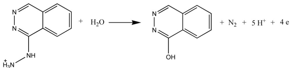
Scheme 2. Proposed electrode reaction of Hy-HCl.
