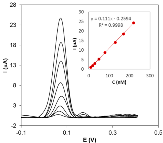
Figure 5. DPVs for a solution containing different concentrations of Hy-HCl (10-220 nM) at MWCNT/GC electrode. Scan rate: 50 \text{ mVs}^{-1} , accumulation time: 120 sec, electrolyte: 0.1 M PBS (pH 7.0). Inset plot shows the linear dependence of current vs. concentration.
