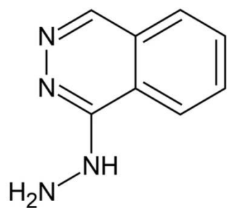
Scheme 1. Chemical structure of hydralazine.
