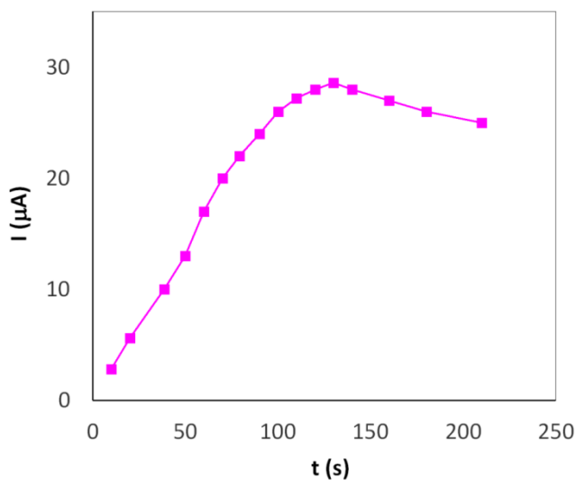
Figure 4. Effect of accumulation time on the oxidation peak currents of 0.22 \mu\text{M} Hy-HCl ( 0.1 \text{ M PBS} , \text{pH } 7.0 ) in open circuit potential.
