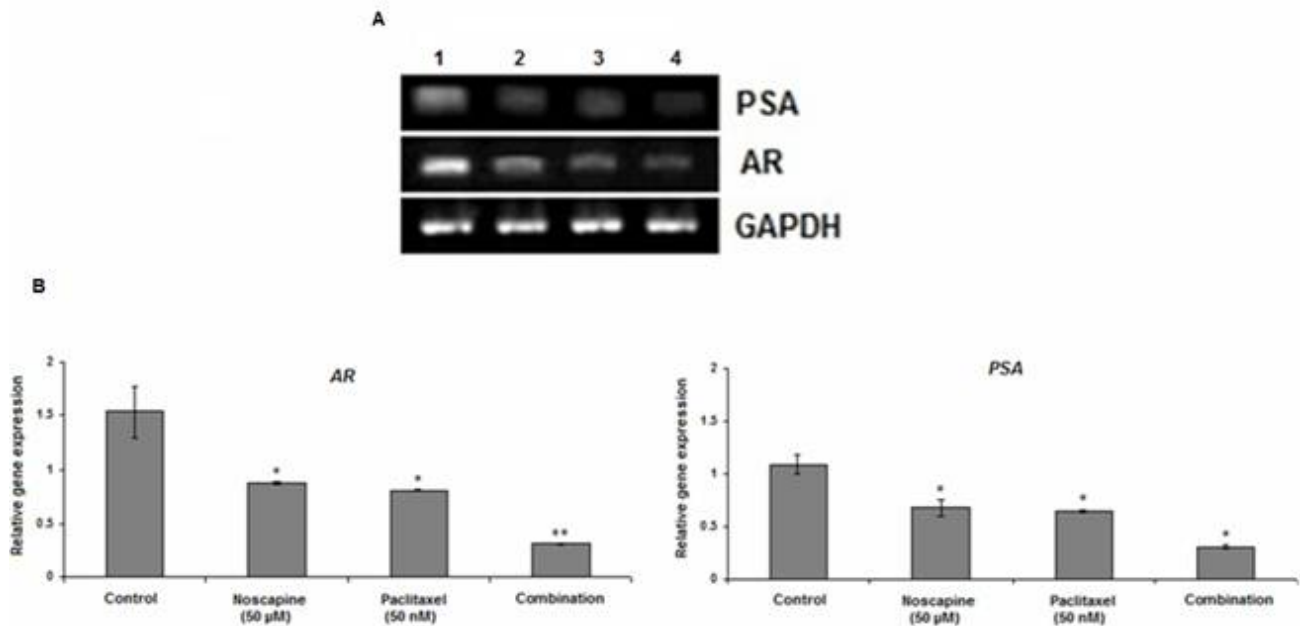
Figure 4. Effect of 50 nM paclitaxel, 50 μM noscaphine and their combination on mRNA
