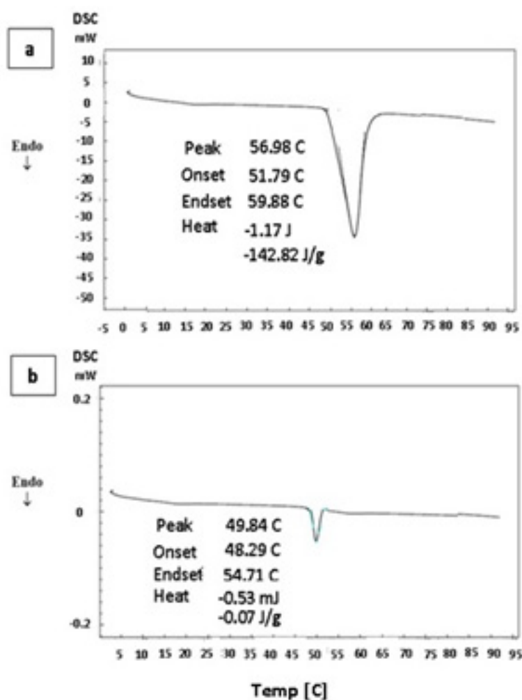
Figure 4. DSC thermograph of thymol (a) and thymol loaded microparticles (b).
