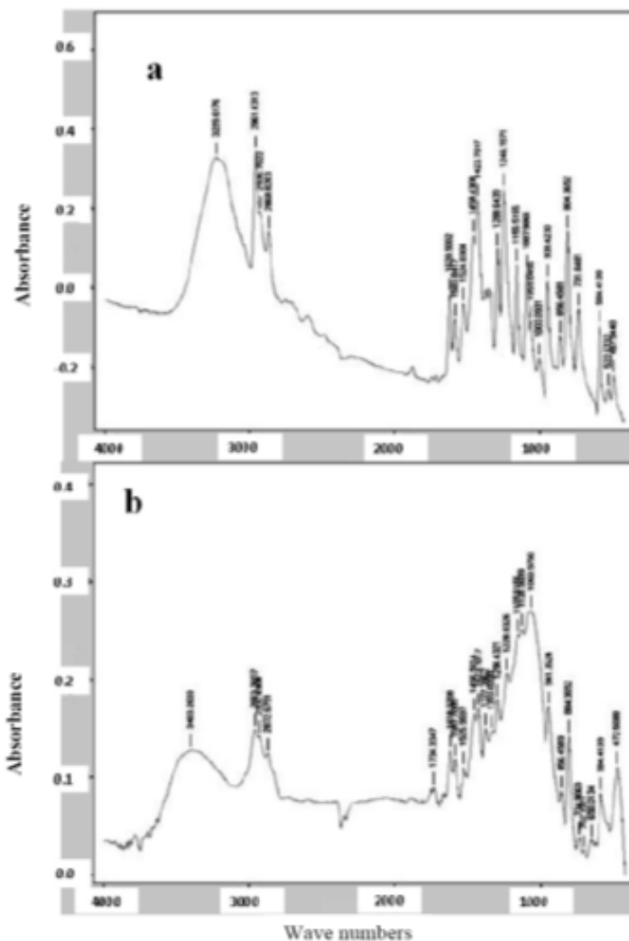
Figure 5. FTIR spectra of thymol (a) and thymol loaded microparticles (b).
