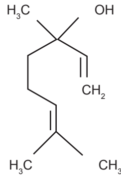
Figure 2. Chemical structure of Linalool as an important constituent of Coriander oil.
