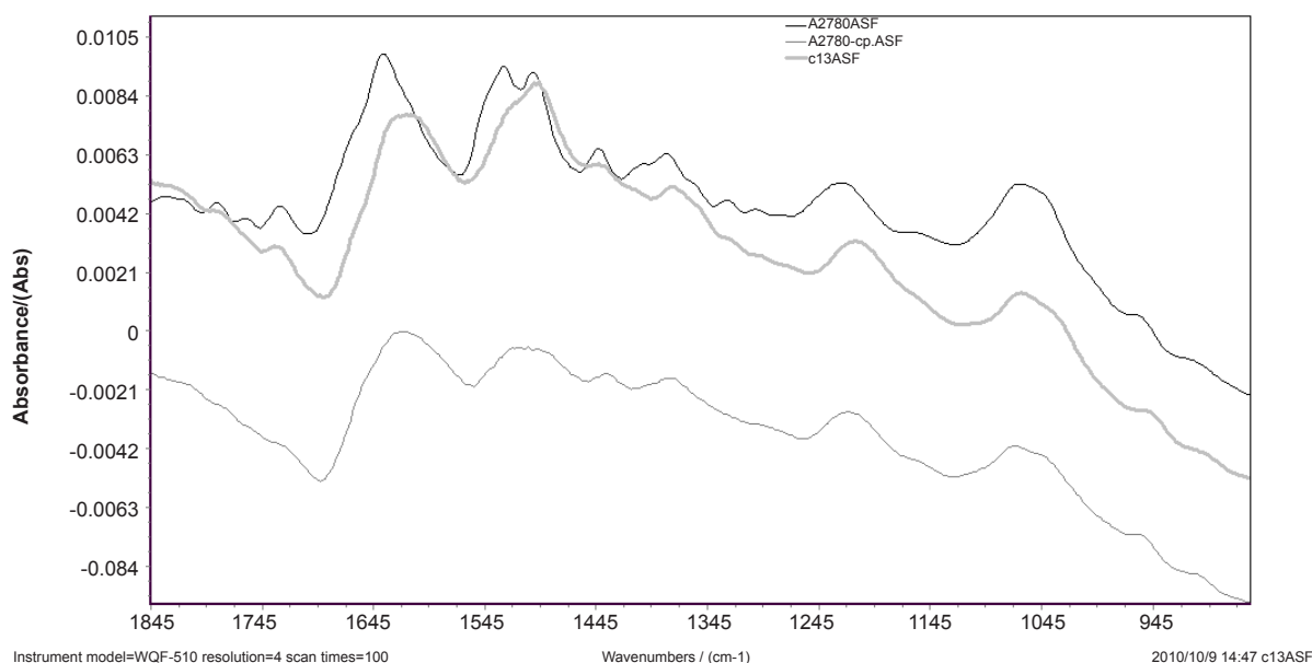
Figure 1. FTIR spectral features of A2780, A2780-CP and C13 cell lines in 1800-900 \text{cm}^{-1} .
